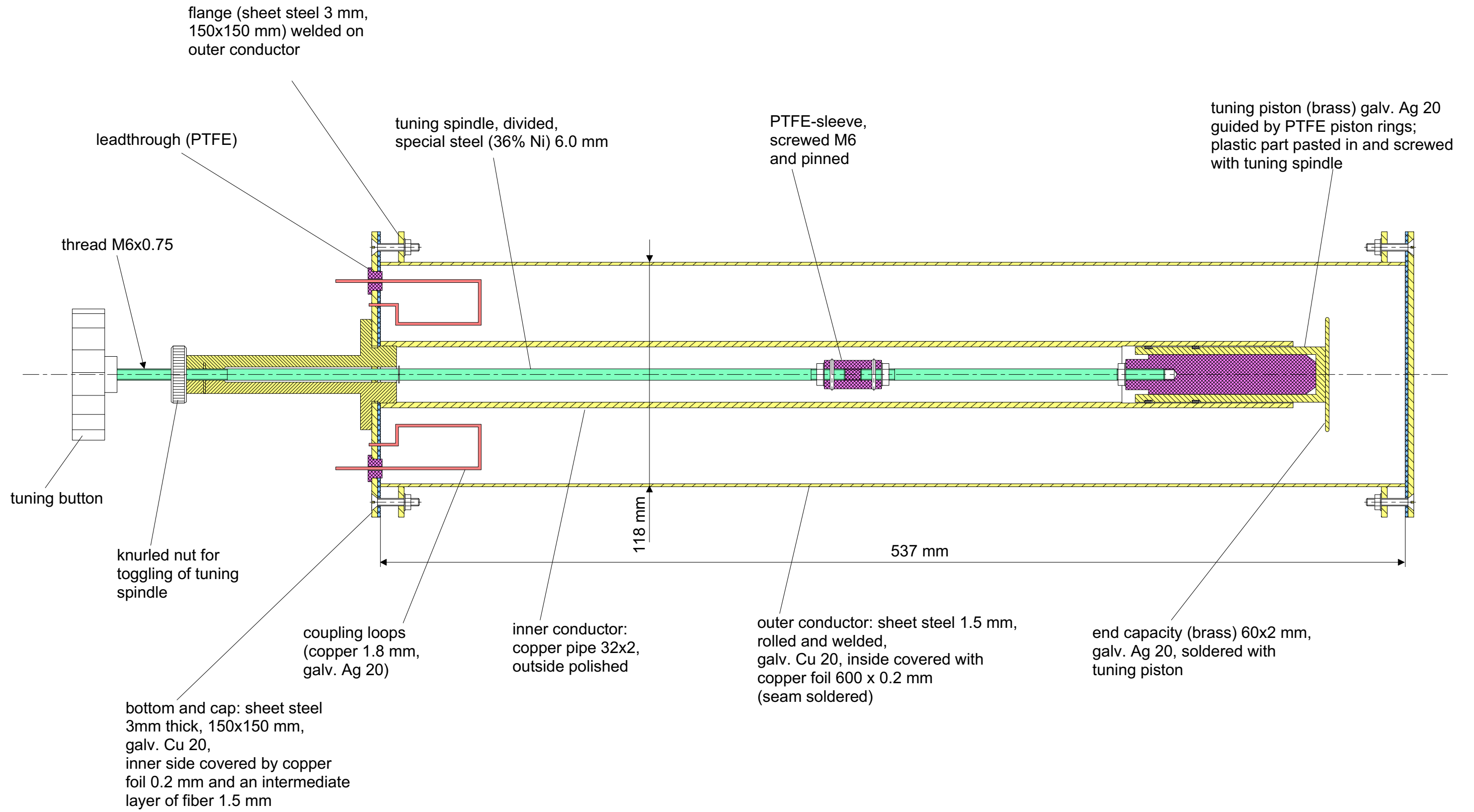
Resonator Cavity for 2m-Duplexer DB0GWD (cross section)
